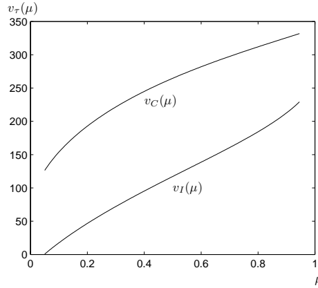
Figure 5: Value functions under free entry ( p_0 = -76 )
